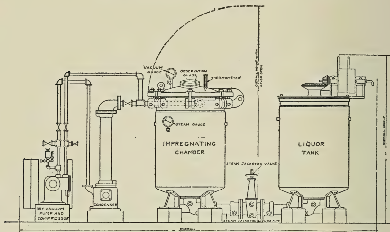
FIG. 149.—Vacuum Impregnating Apparatus.
